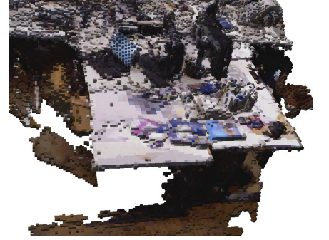
Fig. 3. Using only stepwise tracking leads to undesired results due to the accumulated drift (a). After graph optimization with 5 iterations of g^2o , an excellent alignment of most point clouds is achieved (b). Individual clouds are still slightly misaligned. Through integration of the free-space information these artefact are greatly diminished after computation of occupancy probabilities (c).
