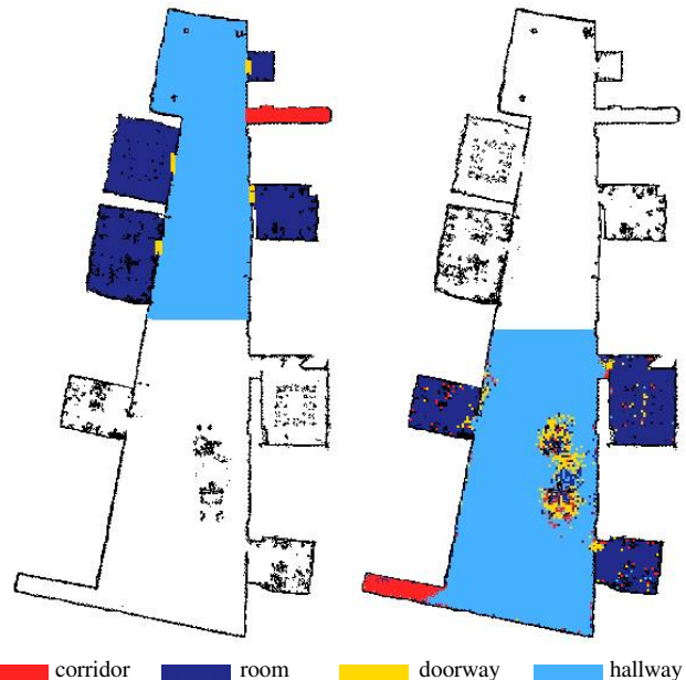
Fig. 6. The left image show the training data used to train the classifiers and the right image the classification results of our sequential AdaBoost classifier.
