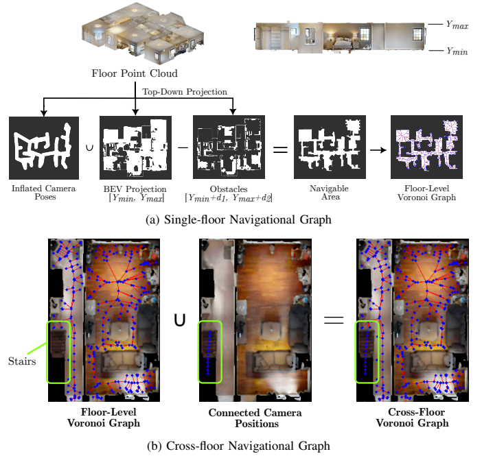
Fig. 5: Actionable navigational graph: The creation of the actionable navigational graph involves constructing single-floor and cross-floor navigational graphs: (a) By deducting the set of obstacles from the union of camera poses and the per-floor obtained BEV projection of the floor point cloud, we obtain the navigable area. Within this area we construct a Voronoi diagram as shown right. (b) In order to equip our navigational graph with cross-floor navigation capabilities, we extract the camera positions within regions classified as stairs . This subgraph is connected with the corresponding floor-level Voronoi graphs.
