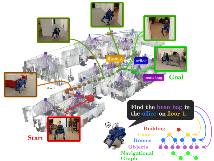
Fig. 1: HOV-SG enables the construction of accurate open-vocabulary 3D scene graphs for large-scale and multi-story environments and enables robots to navigate in them effectively.
