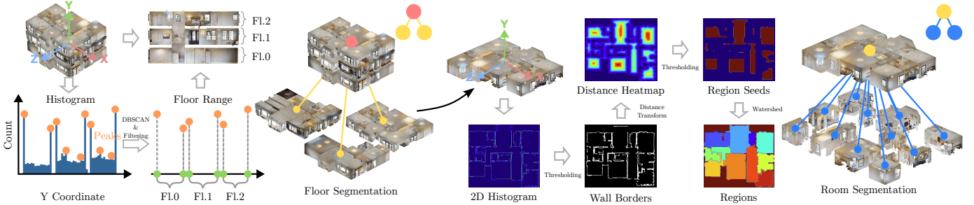
Fig. 3: Floor and Room Segmentation. Given the point cloud of the whole environment, floor and room nodes are subsequently derived based on geometric heuristics. Floor boundaries are computed by finding peaks of the pixel density along the height direction followed by filtering while room segment masks are extracted using the Watershed algorithm.
