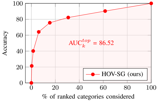
Fig. S.2: We visualize the AUC_k^{top} curve for different evaluation thresholds k , which this plot measures in terms of percent out of the total number of categories (HM3DSem: 1624). The shown curve represents the results of our method HOV-SG on the HM3DSem scene 00824.
