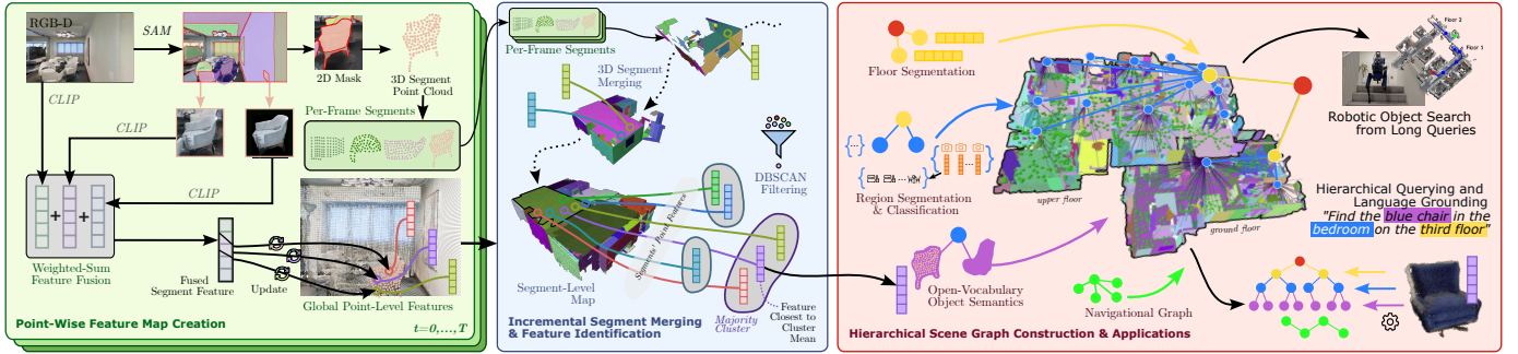
Fig. 2: HOV-SG builds hierarchical open-vocabulary 3D scene graphs of indoor household scenes. We first use SAM to extract object masks per frame while obtaining vision-language features via CLIP. In the next step, we aggregate these features on a point level in the map. Secondly, we segment the full point cloud based on merged 3D masks. To generate more meaningful semantic object features, we employ a DBSCAN-based filtering approach to obtain a majority vote feature for each object. To construct an actionable 3D scene graph, we segment the obtained panoptic map into multiple floors, segment and classify distinct regions using several view embeddings, and identify object names via querying. As a result, HOV-SG allows hierarchical querying and navigation using mobile robots even in complex multi-floor environments.
