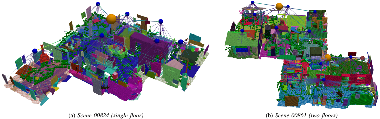
Fig. 7: Qualitative visualization of the hierarchical 3D scene graphs produced by HOV-SG of two apartments of the Habitat Matterport 3D Semantics dataset [25]. Yellow nodes represent floors, while blue nodes represent rooms. The green graph right above the respective floor represents the produced navigational graph. For more visualizations, please refer to Fig. S.4.
