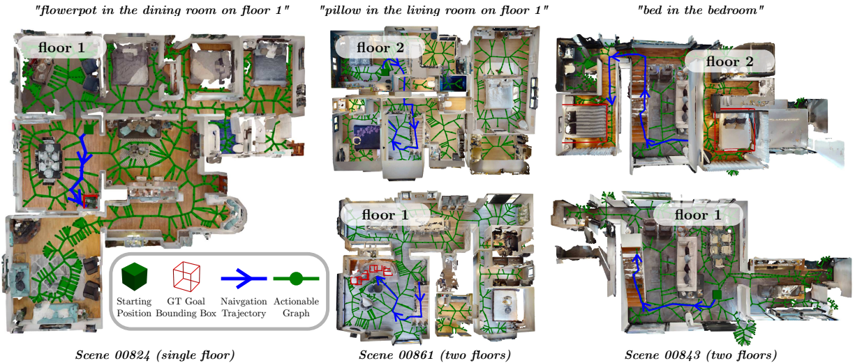
Fig. 8: Qualitative visualization of the language-conditioned navigation in multi-floor environments in HM3DSEM dataset. In some cases, there are multiple ground truth objects matching the instruction. Stopping at any of them with a distance within 1 meter is regarded as a success.
