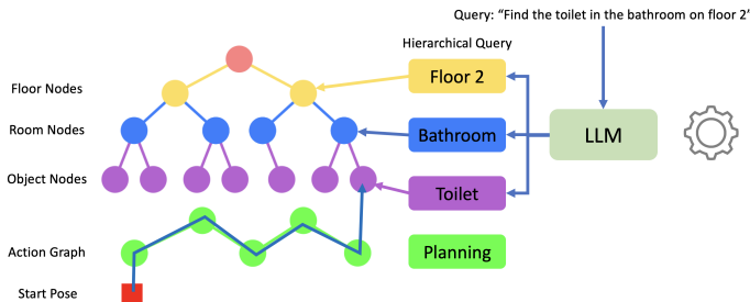
Fig. S.1: The language-grounded navigation module of HOV-SG allows to parse complex queries such as “find the toilet in the bathroom on floor 2” into three queries using a large language model (GPT-3.5) - one each for the floor, room, and object levels. Leveraging HOV-SG’s hierarchical structure, we progressively narrow down the search space by querying at each level. Once the target location is identified, the action graph in HOV-SG is used to plan a path from the starting pose to the target.
