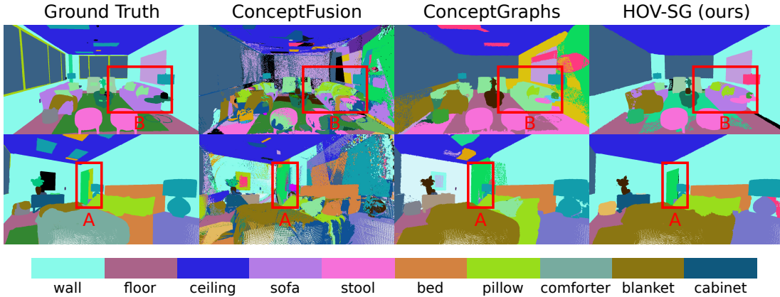
Fig. 6: Qualitative results for 3D semantic segmentation on Replica dataset. For conciseness, the legend only shows ten out of 101 categories in the Replica dataset. Observing the position “A” indicated in the images, only HOV-SG predicts the door with correct boundaries. At position “B” in the images, only HOV-SG predicts the sofa correctly.
