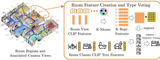
Fig. 4: Room embedding computation and room type voting. We enrich each room node with open-vocabulary embeddings by associating the observations with it. Given the segmented room region and the contained camera poses we extract 10 distinct CLIP features that represent the semantic distribution of a room.
